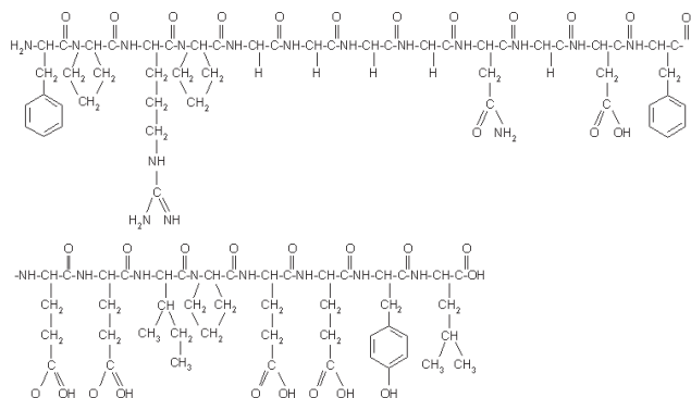
Figure 1. Structural Formula for Bivalirudin
